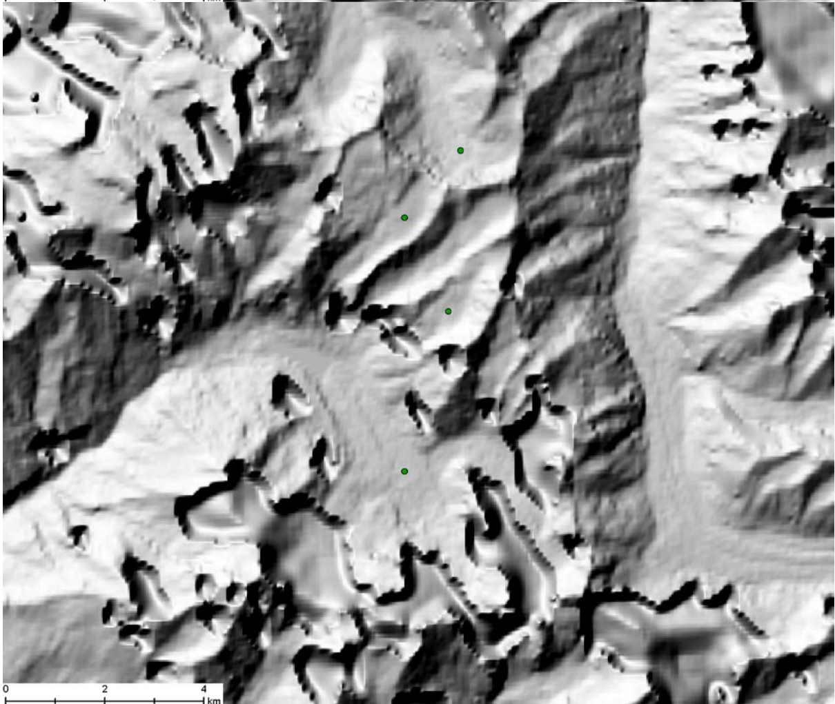
Hillshade of SRTM
