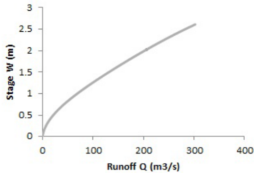
Figure 1 Example of a stage-discharge relationship
