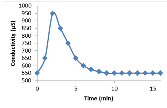
Figure 12 Measurement of conductivity at sampling site after injection of a “gulp” of salt dilution. The time was set to zero when the dilution was arrived at the sampling site.
