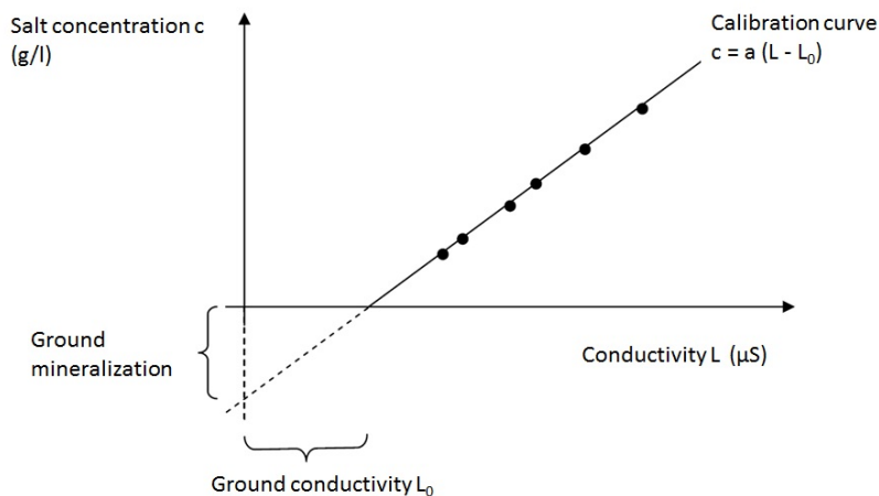
Figure 8 Salt concentration in function of conductivity
