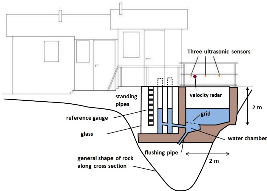
Figure 14 Crosssection of measurement principle at Vernagtbach gauging station. (Bergmann & Reinwarth, 1976)
