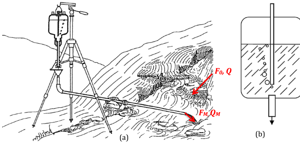
Figure 9 (a) Installation of a Mariotte's bottle and (b) schematic of a Mariotte's bottle
