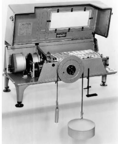
Figure 5 Continuous recording water-stage recorder with cover raised. The time element rotates the rolls, and the height element records parallel to the axis of the rolls ( www.usbr.gov )
