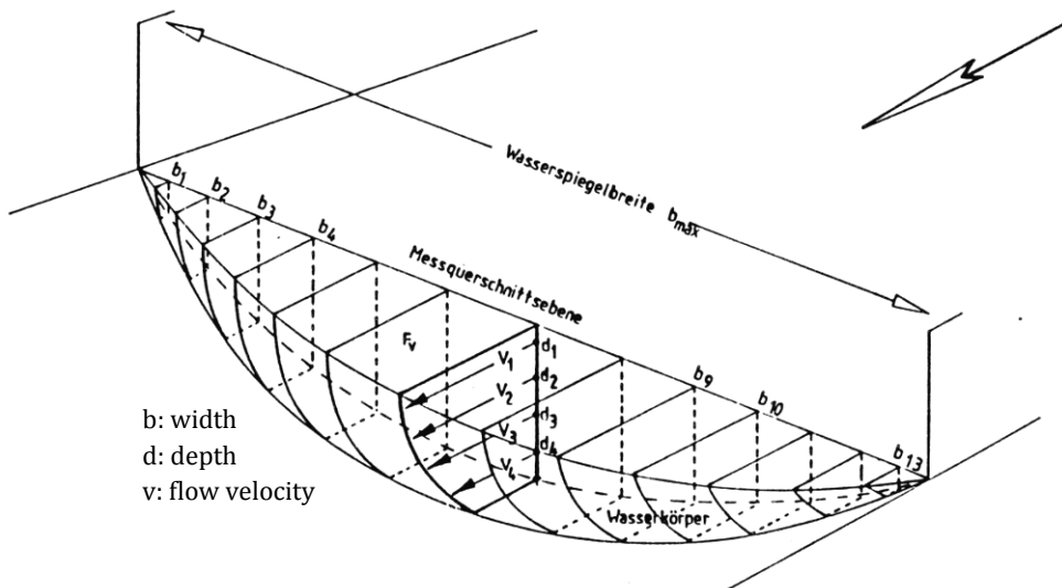
Figure 6 Technique of runoff measurement with a current meter (Landeshydrologie, 1982)
